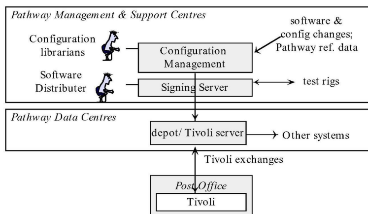
Figure 8-8 Software Release
