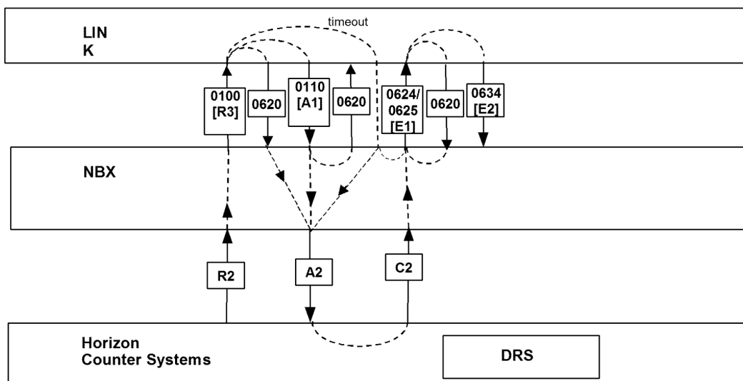
Figure 2 - LINK Message Flows for PIN Change
