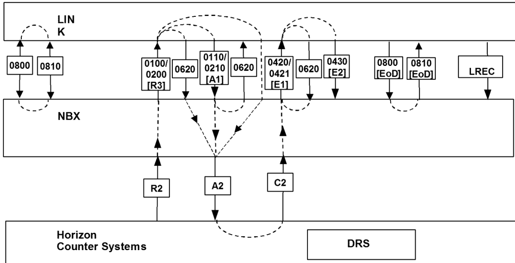
Figure 1 - LINK Message Flows in the Network Banking Environment
