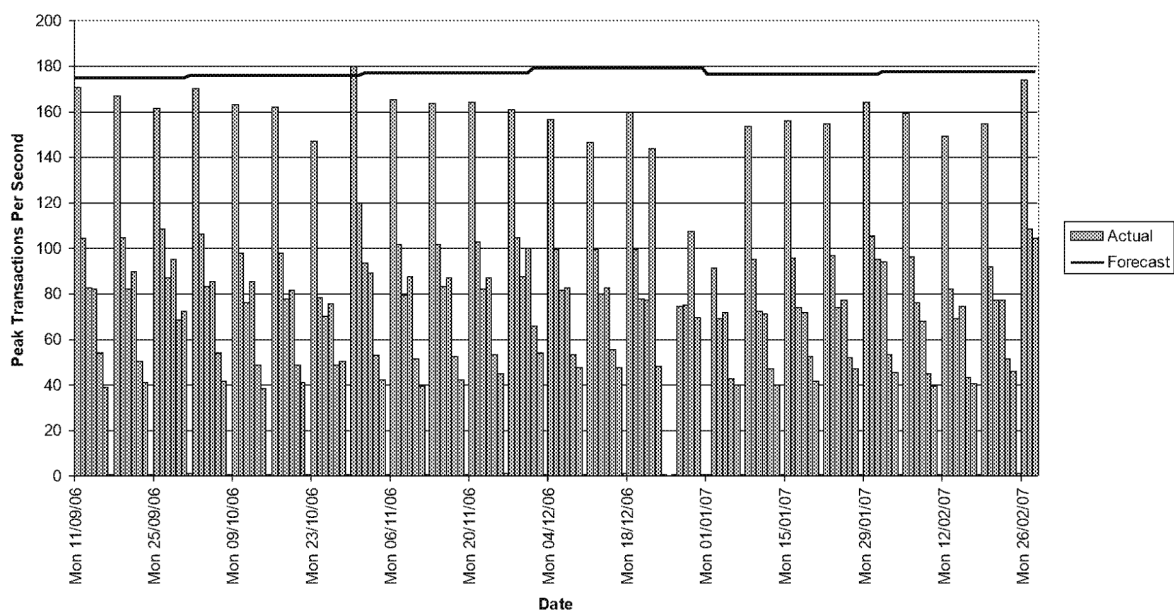
Peak Online Transactions Per Second (Total of NBS, DCS, ETU, DVLA Online, PAF and APOP)
