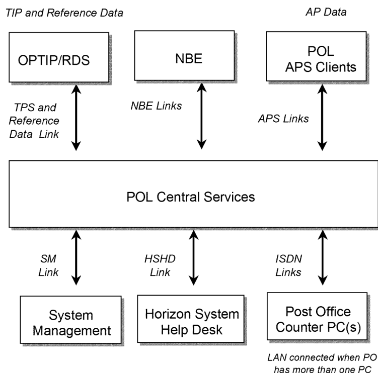
Figure 8.1 Links for Protection
