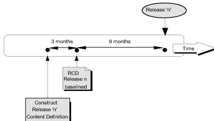
Fig 6.1 - Release Planning
