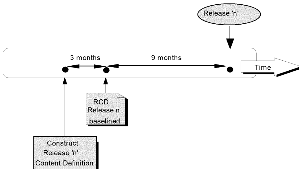
Fig 6.1 - Release Planning
