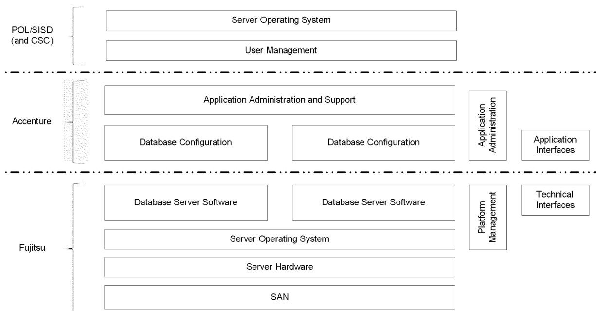
Figure 1: POLSAP Roles
